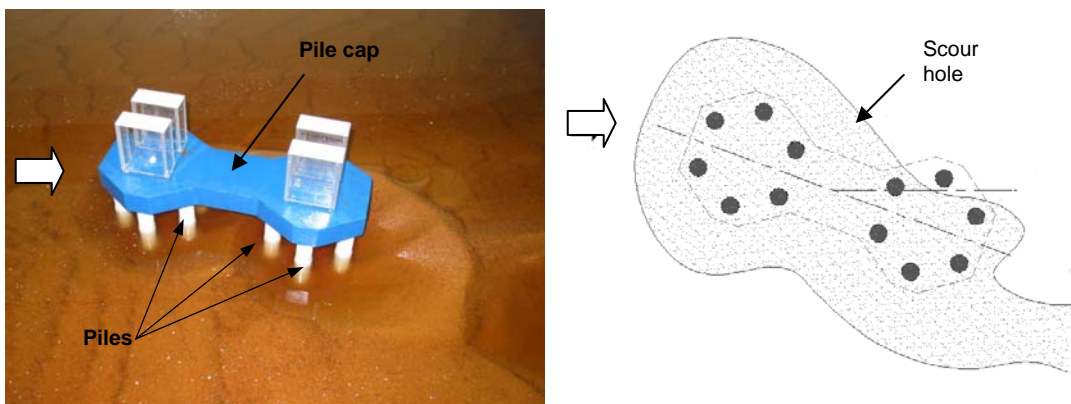
Figure 1. Example of bridge pier with dumbbell-shaped pile cap and hexagonal pile layout, showing also scour hole measured in a physical model.
