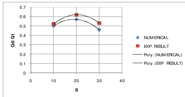
Fig.(12) comparison of experimental and numerical model ( \epsilon = 35\% , Q=25L/S )
