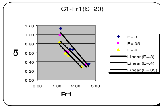
Fig.(9) C_d As function of Fr in slope 30^\circ , \varepsilon = 30\%
